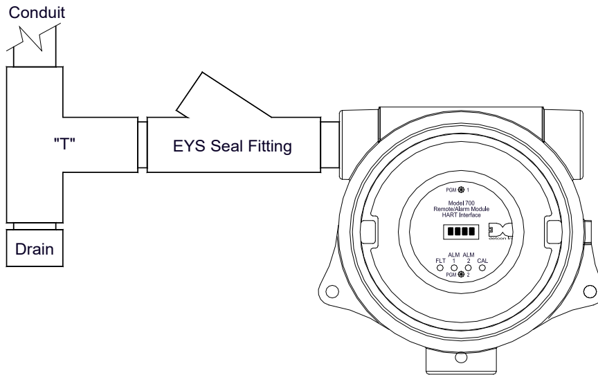
Figure 5 Typical Installation
