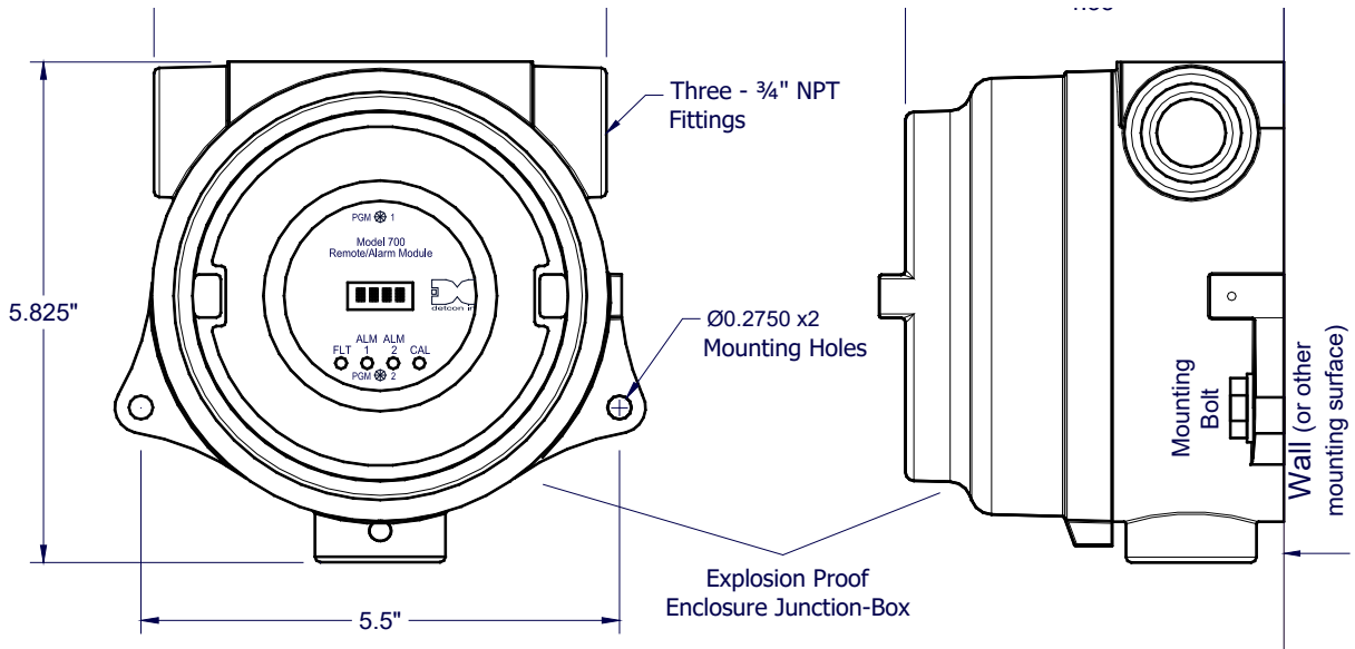
Figure 3 RAM Mounting
