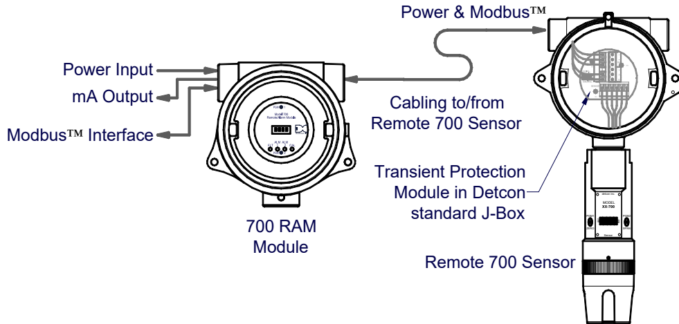
Figure 8 Remote 700 Gas Sensor with RAM
