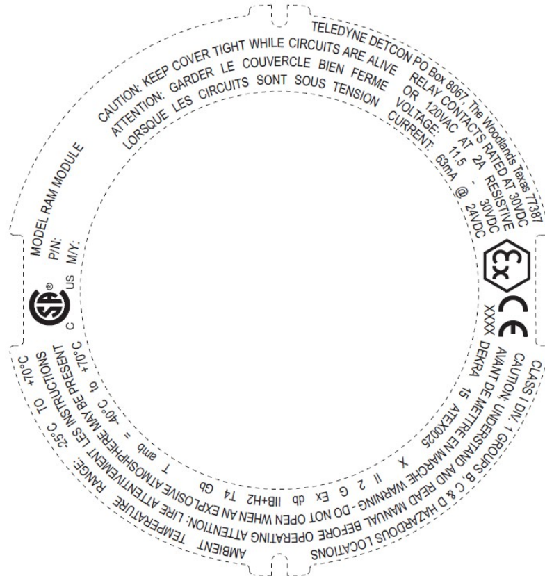
Figure 11 RAM Label
