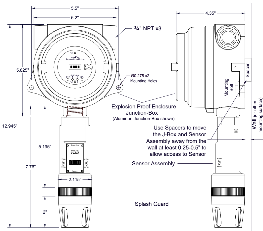
Figure 2 Mounting RAM with 700 Sensor
