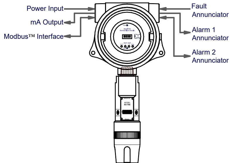
Figure 7 Installation with 700 Gas Sensor
