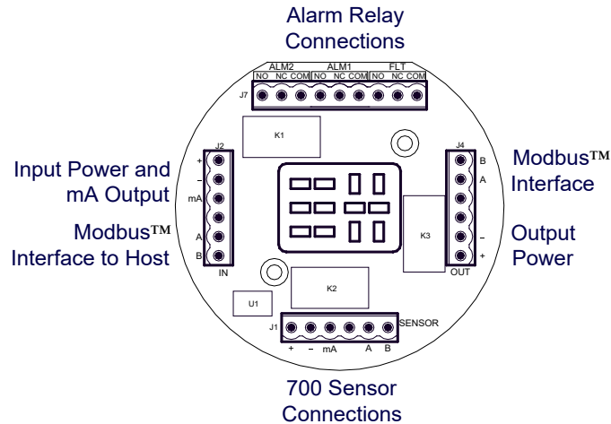
Figure 6 Interface connections on terminal board
