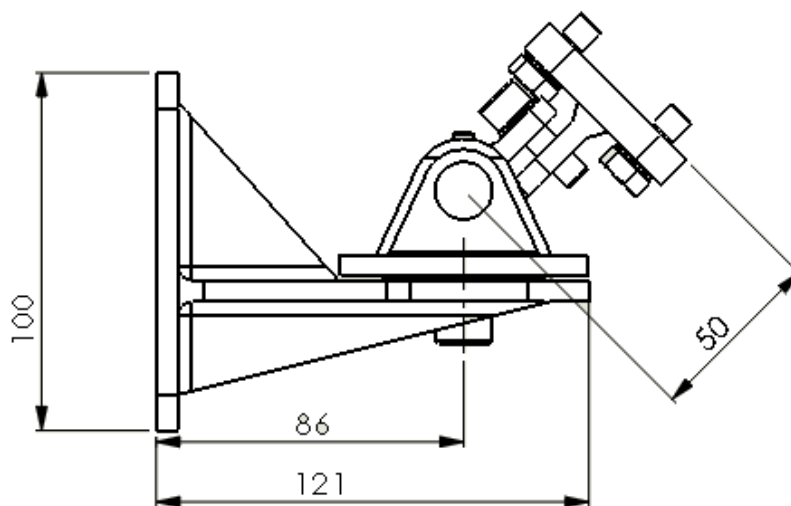
Figure 12: Tilt mount base – Side View
