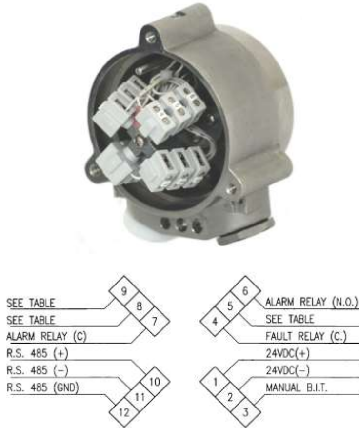
Figure 9: Wiring Terminals
